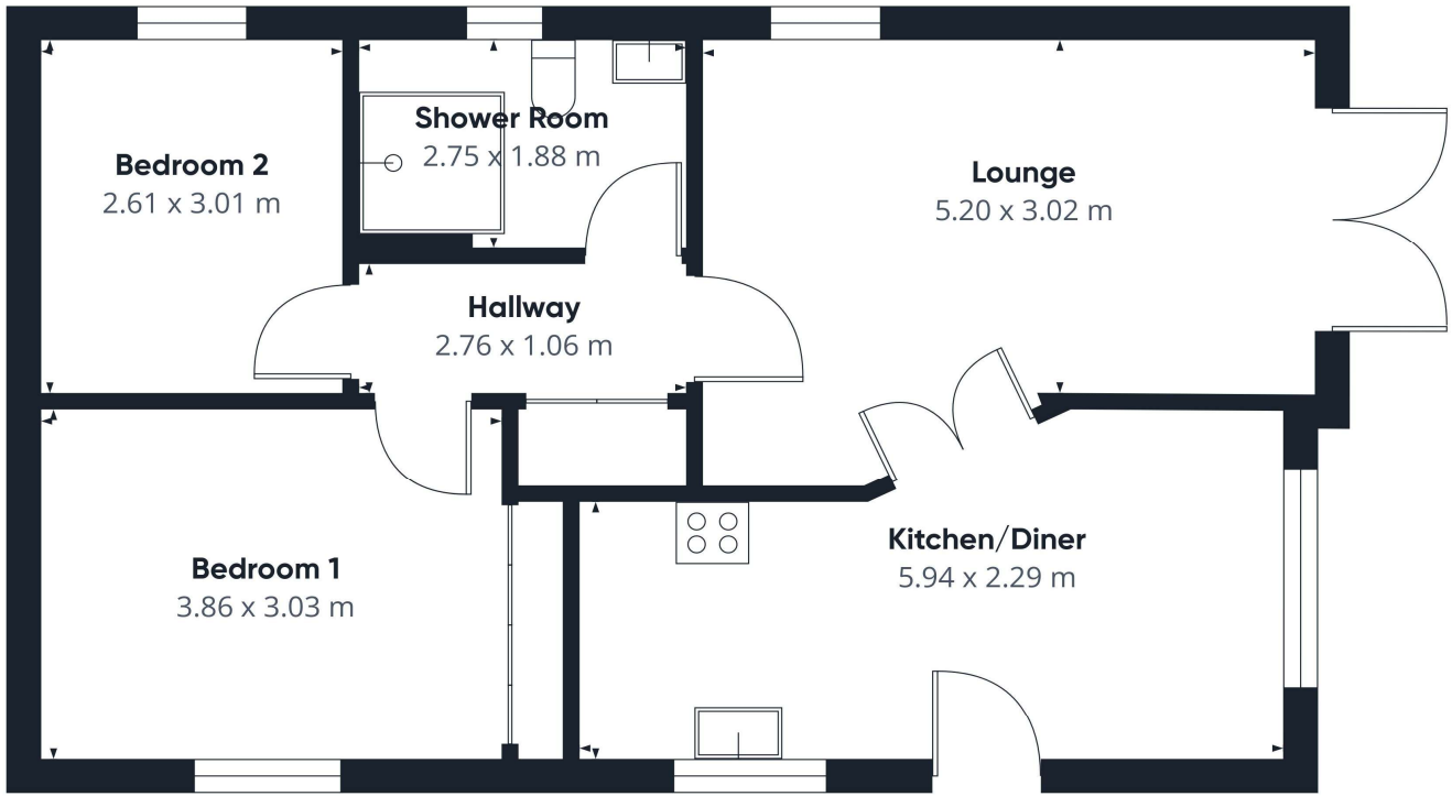
Floor 0 Building 1
